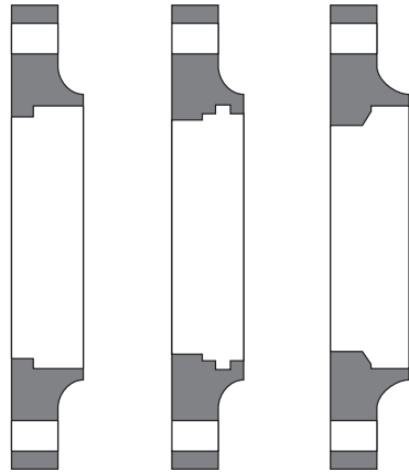
Socket Weld
