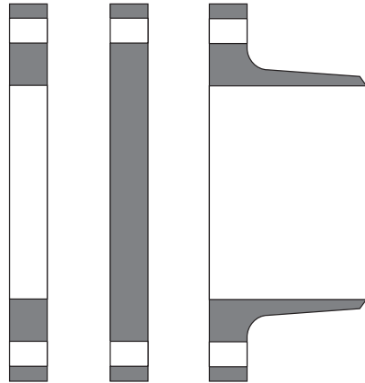
Slip-On
