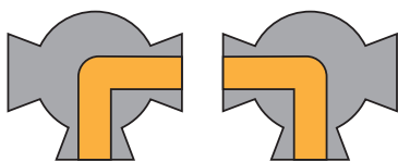
Flow Plan 9: 3 Way, 3 Port, 90° turn, 2 Positions
