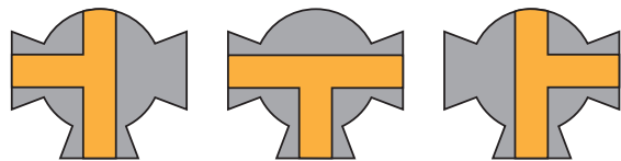
Flow Plan 2: 3 Way, 3 Port, 180° turn, 3 Positions
