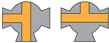
Flow Plan 5: 3 Way, 3 Port, 90° turn, 2 Positions
