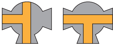
Flow Plan 6: 3 Way, 3 Port, 90° turn, 2 Positions
