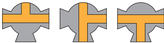
Flow Plan 3: 3 Way, 3 Port, 180° turn, 3 Positions
