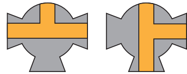
Flow Plan 7: 3 Way, 3 Port, 90° turn, 2 Positions
