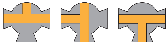
Flow Plan 4: 3 Way, 3 Port, 180° turn, 3 Positions
