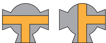
Flow Plan 8: 3 Way, 3 Port, 90° turn, 2 Positions
