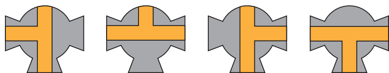
Flow Plan 10: 3 Way, 3 Port, Without Stop Ring, 4 Positions
