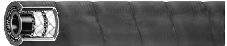
MIL-H-24136/3 EQUAL TO AEROQUIP P/N 2580
